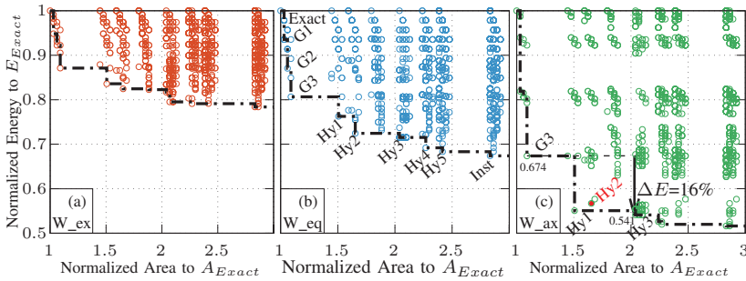
Fig. 4: Design space of an accuracy configurable Sobel Filter under 3 different utilizations given in Table I. Pareto solutions in Figure 4b are labeled to be used in Figure 5.
