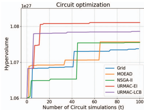
Fig 5: Results of different multi-objective algorithms including URMAC. The hypervolume metric is a function of the number of circuit design simulations.
