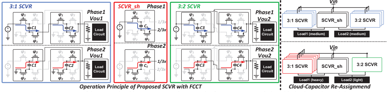
Fig. 1. Power stage of the proposed multi-output SCVR and an example of two-output SCVR design with cloud-capacitor technique.
