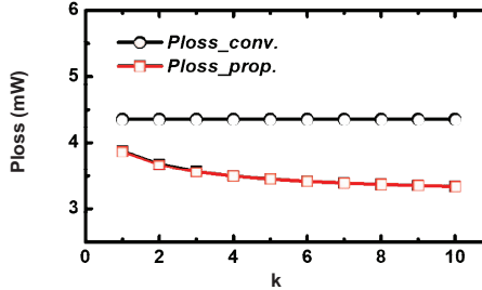
Fig. 3. Relationship between the power loss ( P_{loss(S)} ) and k . Comparison between the conventional and the proposed approach when I_1=I_2 .
