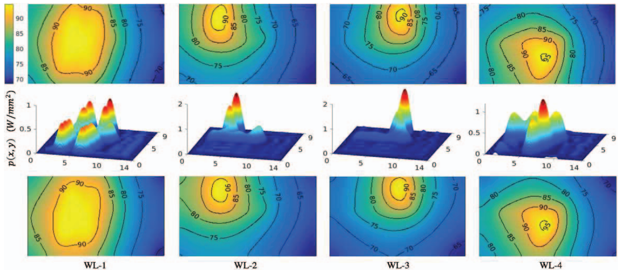
Fig. 9. The power map estimation results, from first to last row are experiment measured thermal maps, estimated power maps in 3D view, and simulation generated thermal maps, respectively. Each column is related to one workload at one steady state.
