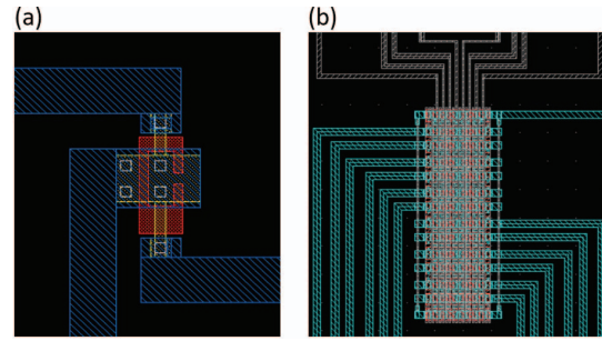
Fig. 6. Layout of a (a) single Y-flash cell (b) 12x8 memristive array. These layouts were checked using DRC and LVS.
