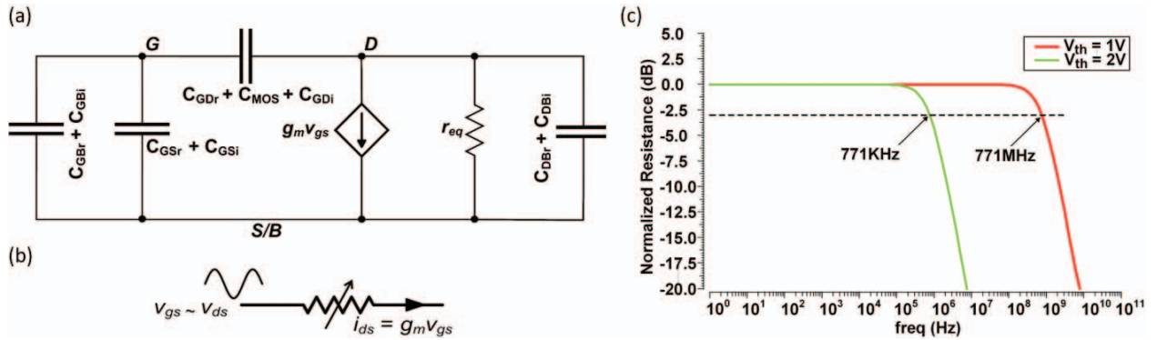
Fig. 4. (a) Subthreshold small-signal schematic of the Y-flash device developed from two parallel-NMOS and parasitic transistors. Since the two NMOSs have the same terminal voltages, they can be folded to develop a single schematic in parallel. Note: C_{GD} \gg C_{GS} . (b) An approximate small-signal schematic of the Y-flash (passive) device. (c) 3-dB frequency range, which demonstrates the maximum frequency up to which the Y-flash device works as a linear resistor in response to small-signal changes.
