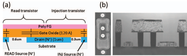
Fig. 1. (a) Single poly Y-Flash device cross-sectional structure in a standard CMOS process, using two NMOS transistors, with asymmetrical coupling gate-drain to gate-source capacitance ratio, where the gate-drain capacitance is made larger. (b) SEM photography of the Y-Flash device: top and cross-section view.
