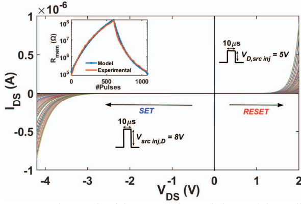
Fig. 3. I-V hysteresis of the proposed memristive model. Reading R_{mem} by a voltage sweep at every state which varies as a function of pulses number for programming voltage of 5V/10\mu s and erasing voltage of 8V/10\mu s . Inset illustrates modeled memristance fitted to the small signal measurements of fabricated DUTs in [9].
