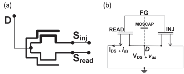
Fig. 2. (a) Schematic symbol of a three-terminal Y-flash. (b) The Y-flash memristive device in read mode, as schematically modeled using three NMOS transistors: parasitic (drain to gate coupling capacitor), read and injection. The current via the injection transistor is negligible in subthreshold.
