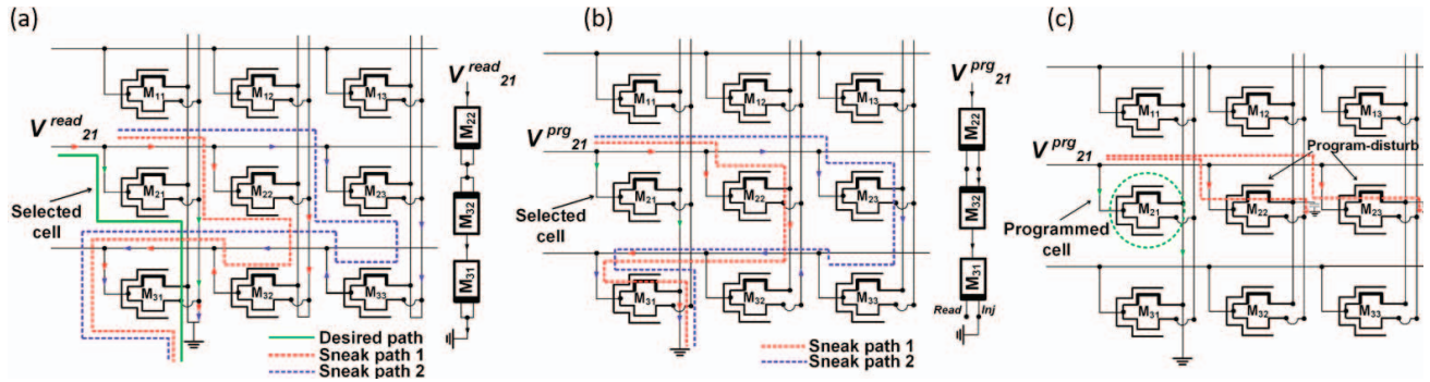
Fig. 7. A 3x3 representative crossbar illustrating sneak currents (a) while reading, and (b) while programming. The insets in (a) and (b) depict the shortest sneak path topology in the array. (c) While programming, the state of the adjacent unselected devices may be disturbed because of substrate leakage current via the injection transistor.
