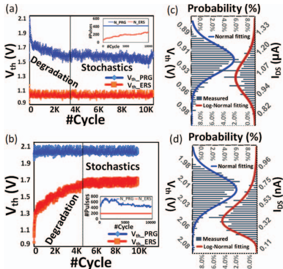
Fig. 5. (a-b) RESET/SET degradation as a result of injected electrons/holes into the floating gate. In the beginning, injection is destructive, and the V_{th} level is decreased/increased under the same number of programming/erasing pulses, while (adaptively) varying the number of pulses to get LRS/HRS, as shown in the insets. (c-d) After the degradation has almost stopped, the measured switching stochastics in [9] are modeled and fitted to normal and log-normal distributions of V_{th} and I_{DS} , respectively in LRS/HRS.
