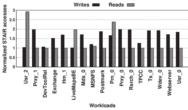
Fig. 5: Reads/Writes of STAIR normalized to the baseline
