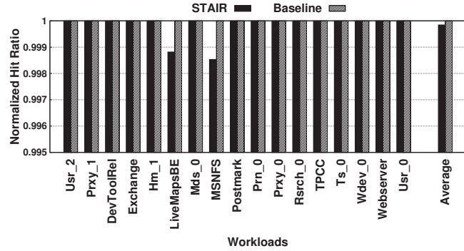
Fig. 7: Hit ratio of STAIR normalized to the baseline
