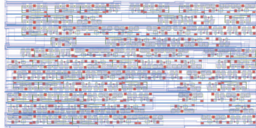
Fig. 1: Layout image of a placed and routed organic thin-film transistor-based 8-bit adder designed with Organic-Flow
