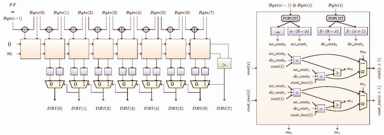
Fig. 5. Hardware architecture of improved DBI encoder
