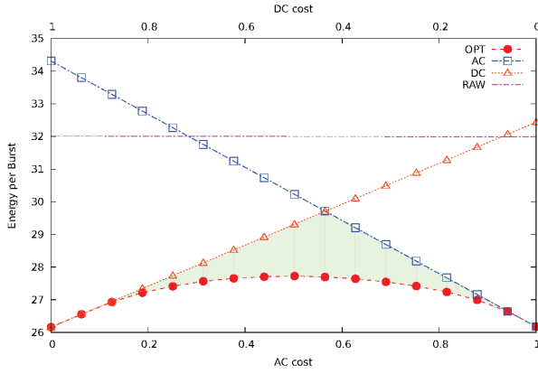
Fig. 3. Energy per Burst using different DBI schemes
