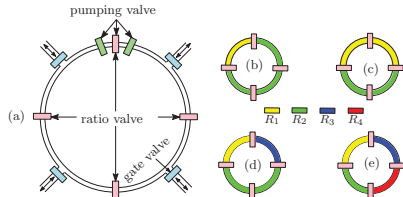
Fig. 2: (a) A 4-segment rotary mixer (Mixer-4) and possible mixing models (b) (1:3) (c) (1:1) (d) (1:2:1) (e) (1:1:1:1)
