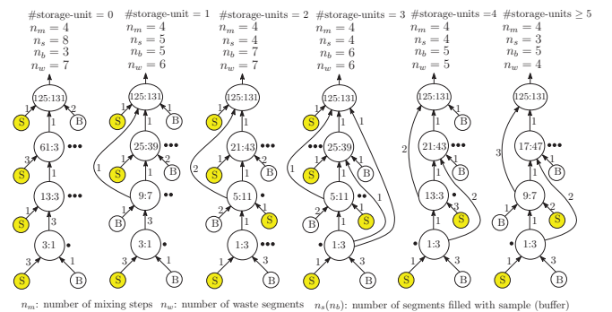
Fig. 9: Reagent minimal solution for the target ratio {sample : buffer = 125 : 131} considering the availability of different number of available on-chip storage-units on the CFMB architecture given in Fig. 1(b)
