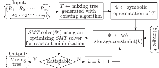
Fig. 6: Flowchart of the proposed algorithm for mixing
