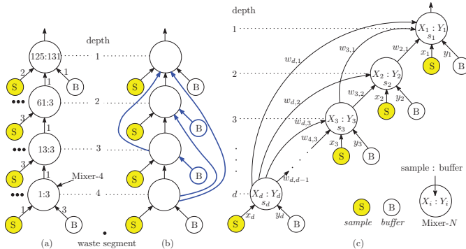
Fig. 7: (a) Dilution tree generated by NWayMix for target ratio {sample : buffer = 125 : 131} (b) dilution graph after adding extra edges and reagent nodes for enabling reagent minimization, (c) general structure of dilution graph
