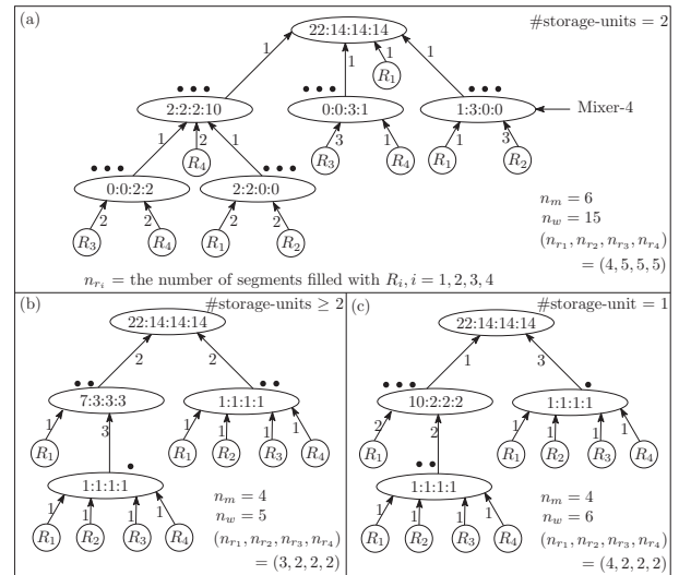
Fig. 11: Mixing tree for the target ratio \{R_1 : R_2 : R_3 : R_4 = 22 : 14 : 14 : 14\} generated by (a) genMixing [7], (b) FloSPA [7] and by the proposed method for \#storage-units \geq 2 , and (c) by the proposed method when \#storage-unit = 1
