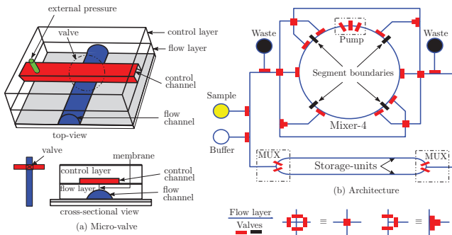
Fig. 1: Schematic of a two-layer microfluidic device: (a) top and cross-sectional view (b) CFMB platform
