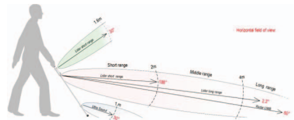
Fig. 3. Obstacles detection of with heterogeneous range sensors.
