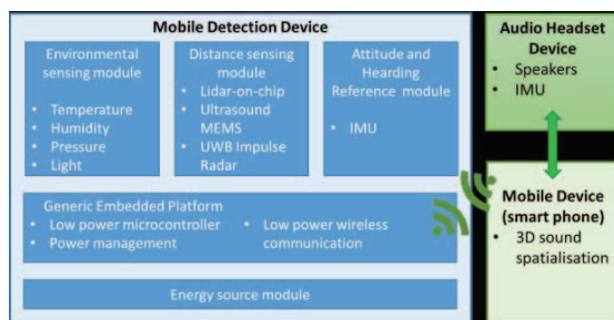
Fig. 5. INSPEX smart integrated system architecture (first attempt).
