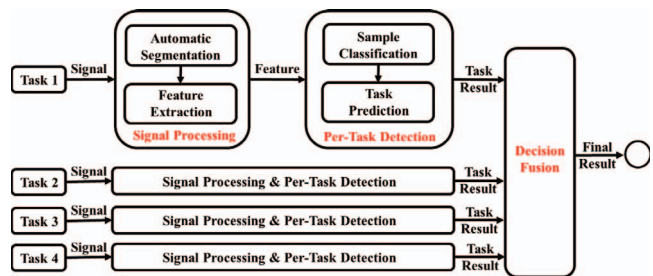
Fig. 4 Computational framework for tunnel vision assessment
