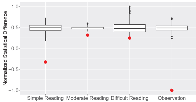
Fig. 6 Difference in standard deviation of feature means of the two groups ('tunnel vision' and 'normal view').
