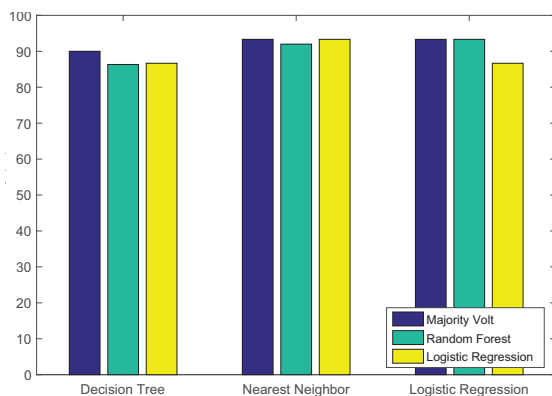
Fig. 7 Accuracy of tunnel vision detection using leave-one-subject-out approach.
