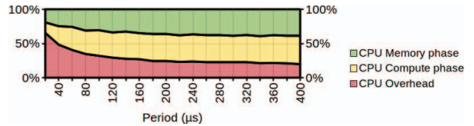
Fig. 3. The division of CPU phases under different period lengths in relation to the CPU synchronization overhead.
