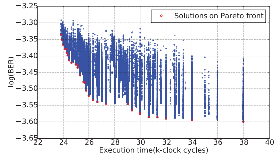
Fig. 7: Valid allocation solutions generated for 8 wavelengths
