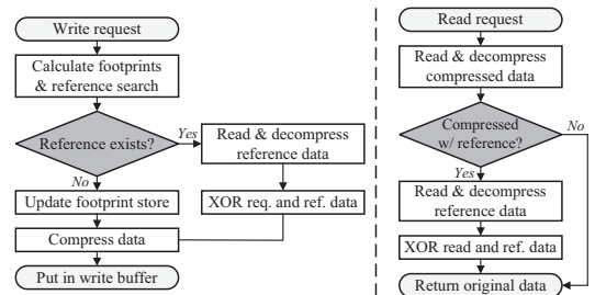
Fig. 3: Request handling procedures of DAC-FTL.
